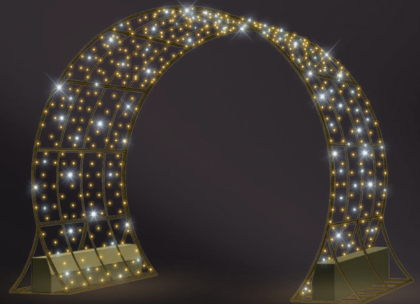
★ Art. No.: I-EBX-07-18-003 600 cm x 400 cm x 80 cm 6.544 LEDs · 436 W · 116 kg
