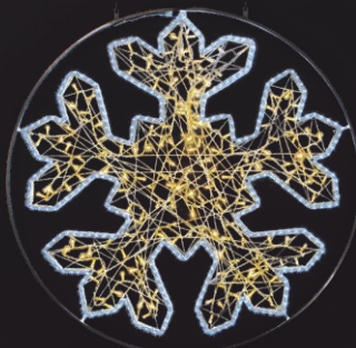
★ Art. No.: 900192LED-WWB0 2D Snowflake, 120 cm · 504 LEDs 26,1 W · 5,7 kg cool-white/warm-white
