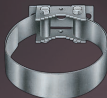
★ Art. No.: MS-2 Universal band clamp for pole mounting from 6 cm diameter.
