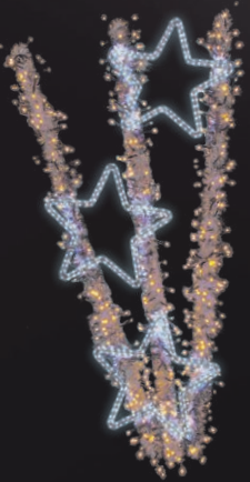
★ Art. No.: 162132109 approx. 110 cm x 210 cm 1026 LEDs · 67,1 W · 10 kg
