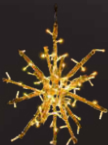
Art. No.: 160520000 110 cm Ø, gold-coloured aluminium, 10,8 W · 24 V · 5 kg
